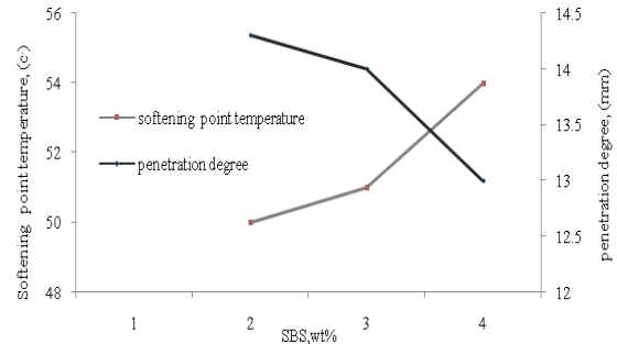
Fig 3. The effect of SBS wt% variations on the SP and the penetration degree (2 wt% bentonite)
