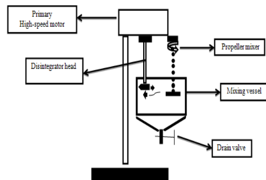
Fig 1: High-speed and high shear double –mixer set
