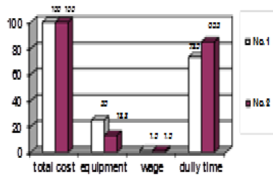
Fig. 3: Contribution of equipment, wage and non-productive time to total cost of No.1 kilns' failures
