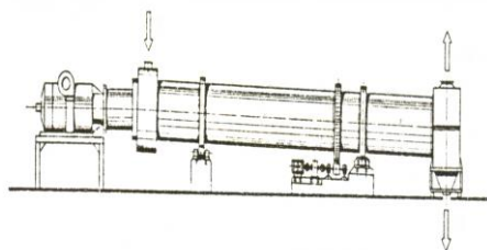
Fig. 1: Construction of longitudinal kiln of company No.1
