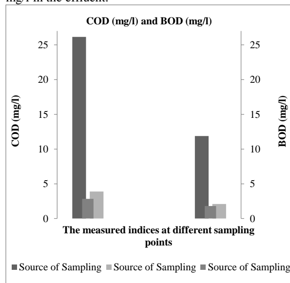
Fig. 3: Six months' mean value of BOD (mg/l) and COD (mg/l) at different sampling points. The standard values of (BOD and COD) regulated by IDE for discharging the effluent to the surface water
