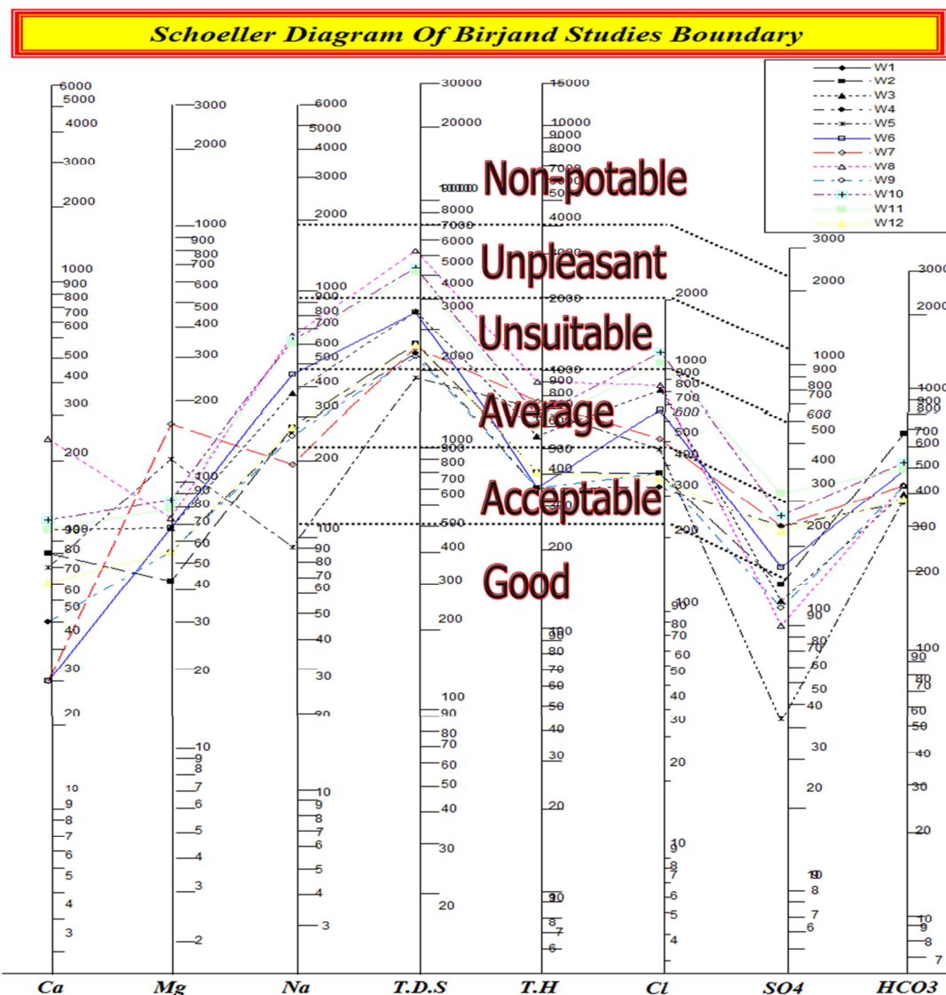
Figure 3. Schoeller diagram of Birjand, Iran flood plain TDS: Total dissolved solids; TH: Total hardness
