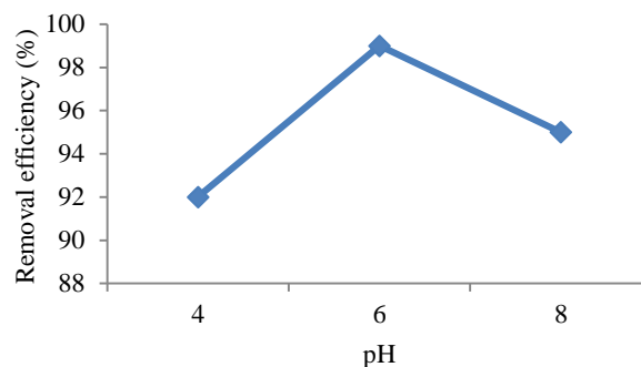
Fig. 4. The removal efficiency based on the pH (the optimum adsorbent level 3 gr and balance time of 3h and optimum adsorbate concentration of 15 mg/l)
