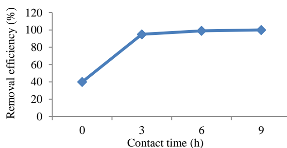
Fig. 2. The removal efficiency in different contact time
