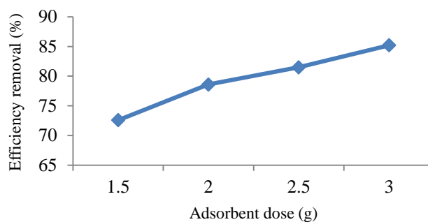
Fig. 1. The removal efficiency based on the various adsorbent concentrations
