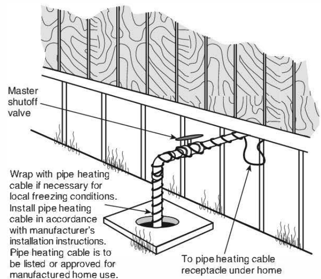
FIGURE A.10.2.3.2 Typical Water Connection.
