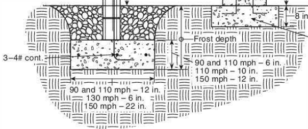
FIGURE 15.5.1.1(b) Masonry/Concrete Foundation Longitudinal Wall and Pier Details.
