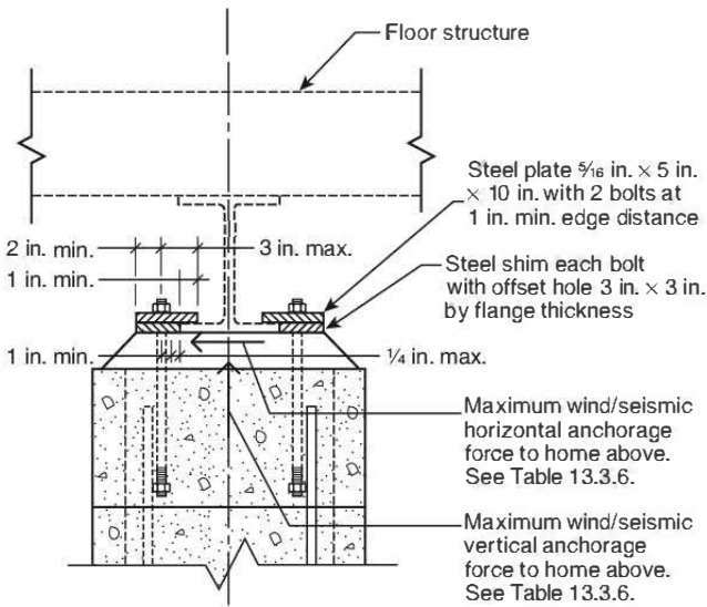
FIGURE 13.3.8 Anchorage Requirements for Shims and Plates.
