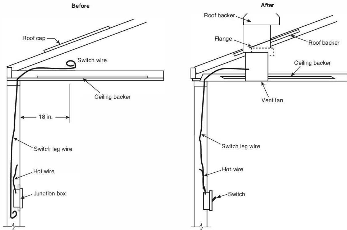
FIGURE A.8.6 Ventilation Improvement Installation.
