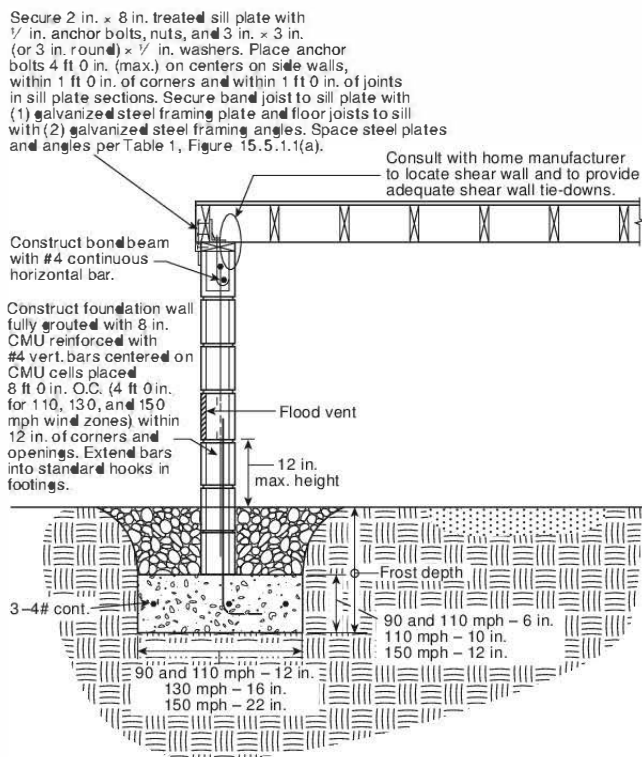
FIGURE 15.5.2(c) Masonry/Concrete Foundation End Wall Detail.
