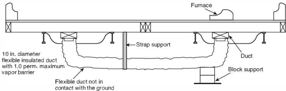
FIGURE 7.4.2.5(a) Crossover Duct Installation (Option 1).
