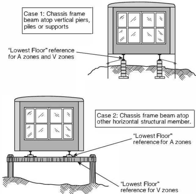
FIGURE A.3.3.19 Lowest Floor Reference for A Zones and V Zones.
