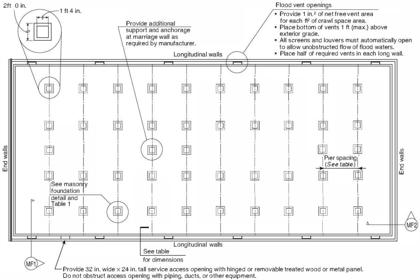
FIGURE 15.5.2(b) Masonry/Concrete Foundation Plan — Double Unit.
