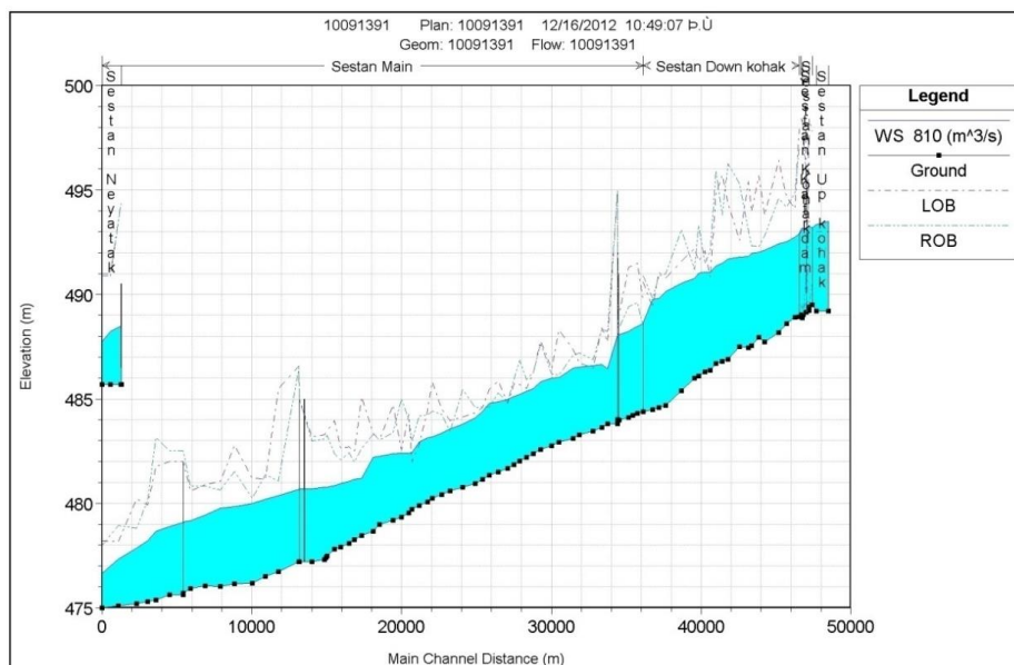
Figure 8- Water Surface Profile in 810 m 3 /s on Lateral with Sistan and Zehak diversion dam
