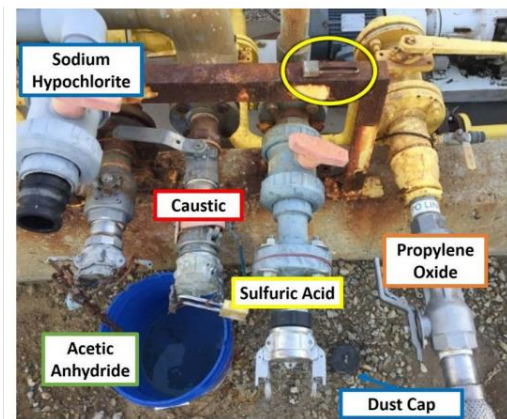
Figure 1: Connections to chemical tanks at MGPI. Sulfuric Acid fill line padlock (circled) on the metal frame. Sodium hypochlorite dust cap on the ground. (ref CSB report 2017-01-I-KS)
